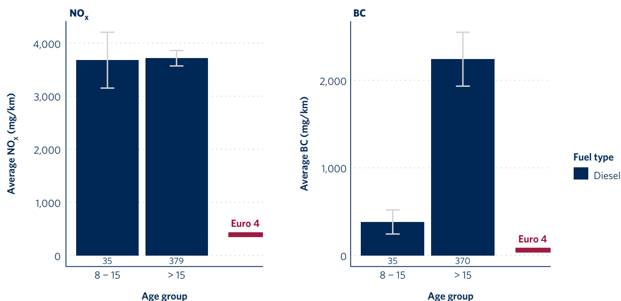
Figure 11. Diesel minibus NO x (left) and BC (right) emissions by age group compared with Euro 4 NO x and PM emission limits of 390 mg/km and 60 mg/km, respectively
