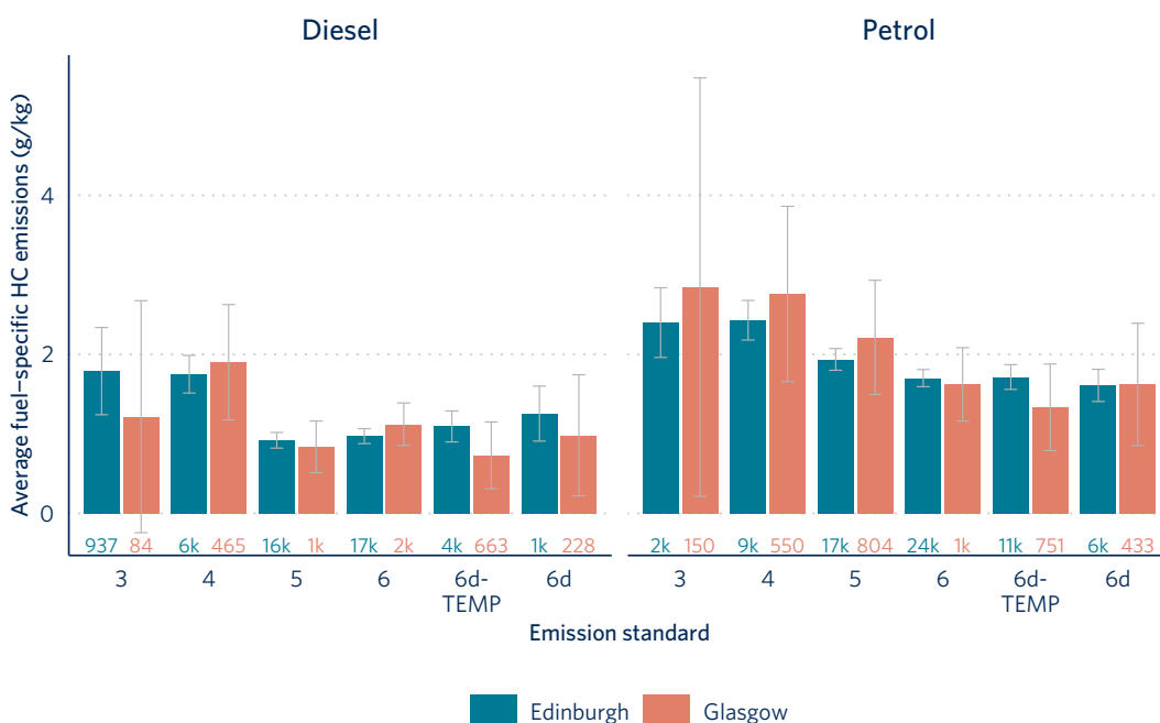
Figure 14. Mean fuel-specific HC emissions from private passenger cars measured in Edinburgh and Glasgow in 2021. The number of measurements is presented below each bar and only measurements of over 50 are presented. Whiskers represent 95% confidence interval of the mean.
